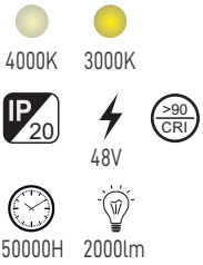
LENSLİ MAGNET ARMATÜR MX-4505
