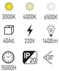
LED RAY SPOT MX-3088
