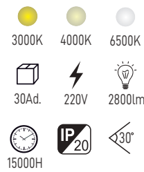
LED RAY SPOT MX-3090
